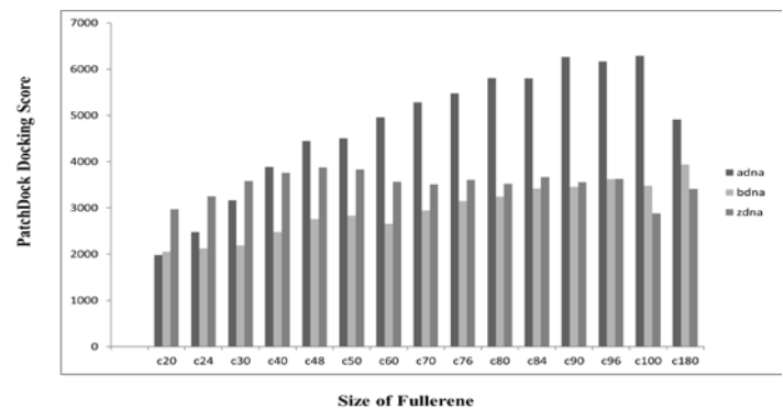
FIGURE 2: Effect of increase in molecular size of fullerene on the docking score with different forms of DNA
