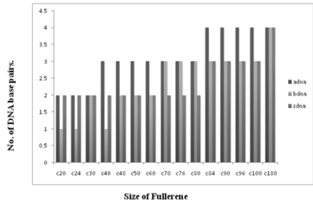
FIGURE 1: Effect of increase in molecular size of fullerene on the number of interacting DNA base pairs.
